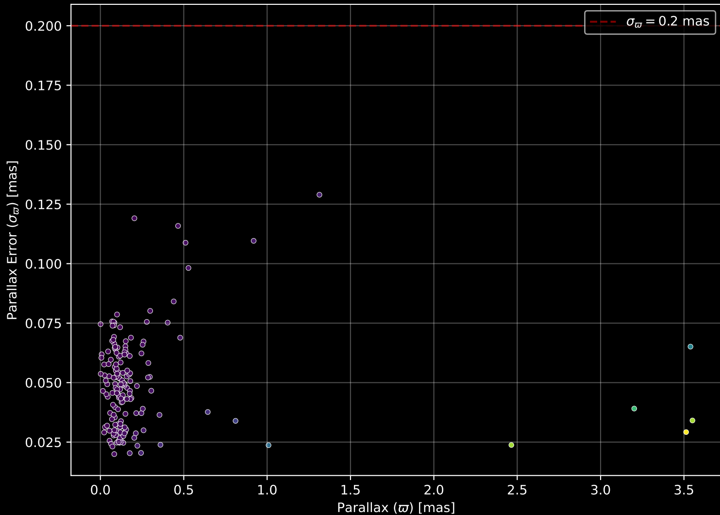
APOGEE DR17 Field: [356-06-O] Parallax Quality (n= 166)
