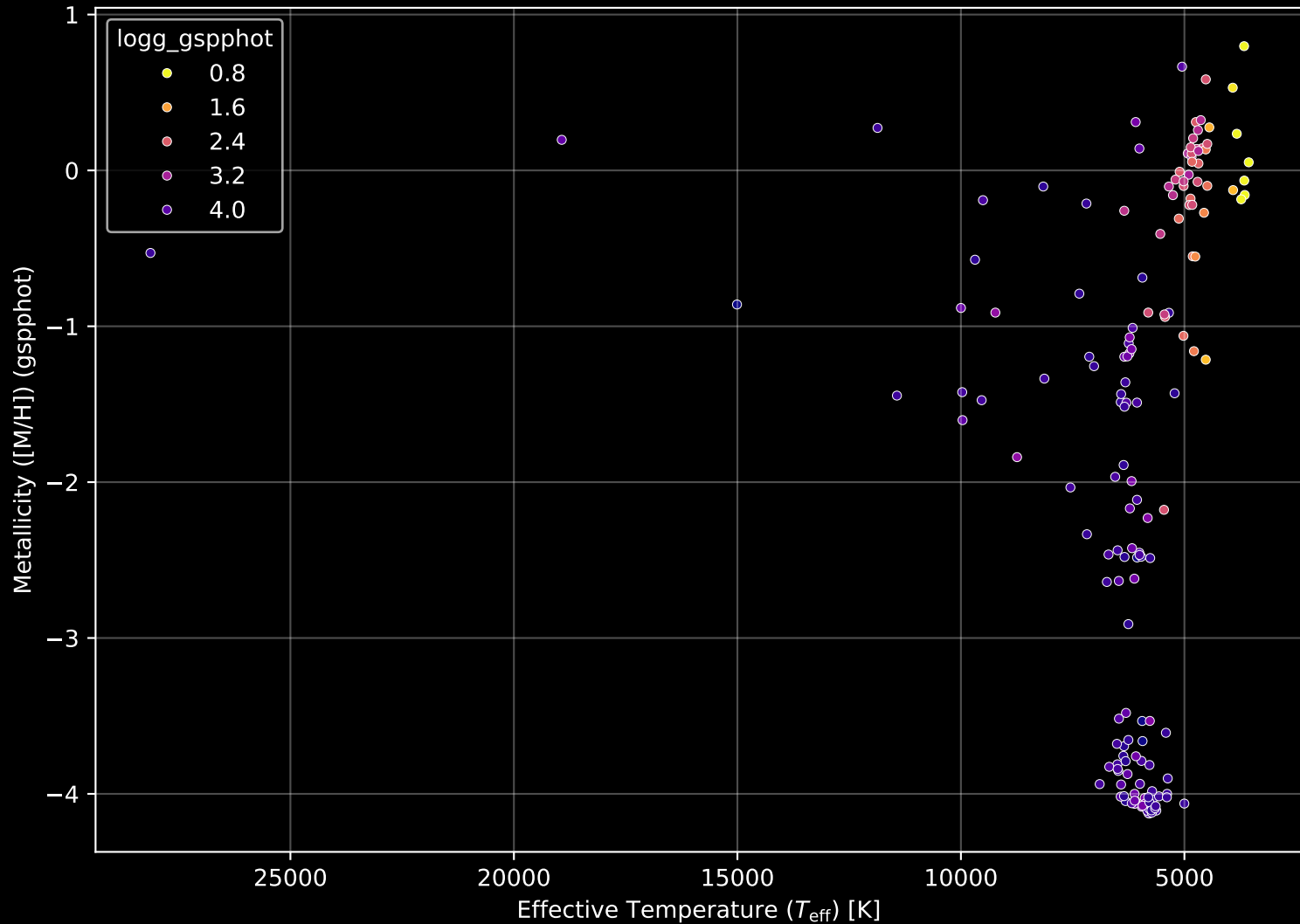
APOGEE DR17 Field: [356-06-O] Stellar Population Parameters (n= 166)
