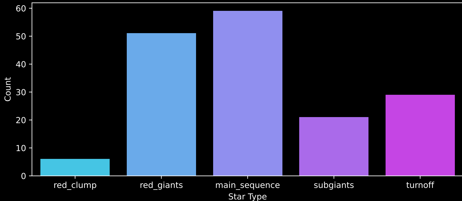
APOGEE DR17 Field: [356-06-O] Count plot of Star Type
