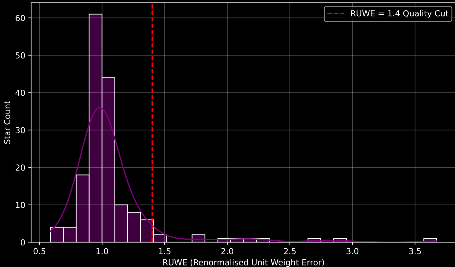
GAPOGEE DR17 Field [356-06-O] RUWE Distribution (n= 166)
