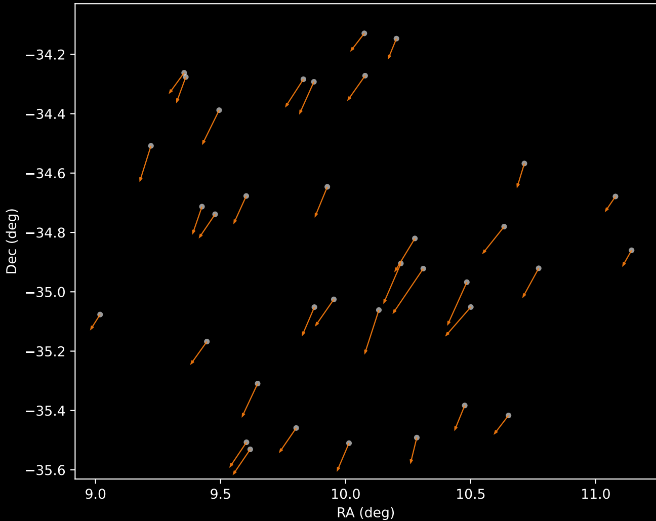
APOGEE DR17 Cluster 2 Proper Motion Vectors (n=36)
