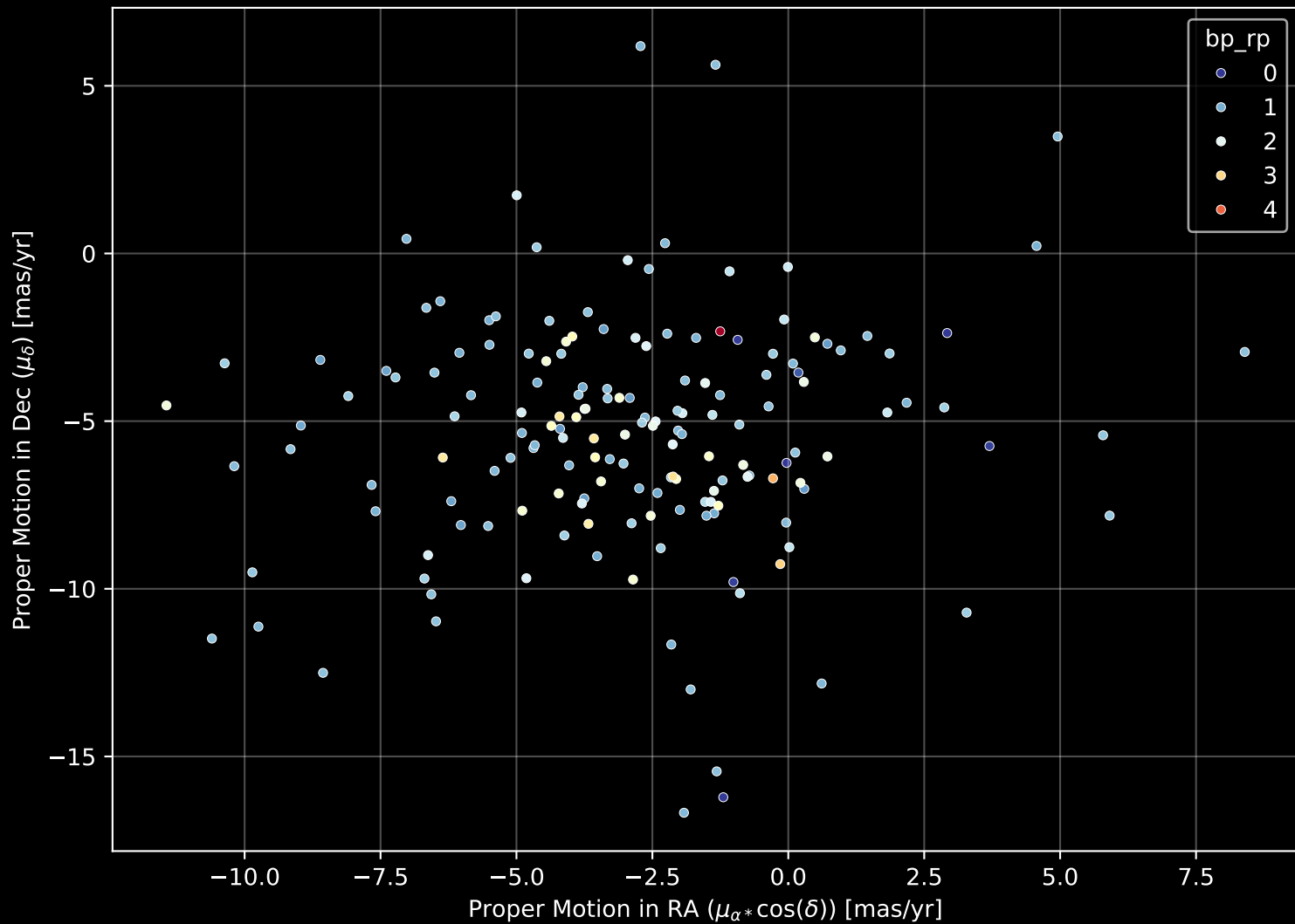
APOGEE DR17 Field: [356-06-O] Proper Motion Diagram (n= 166)
