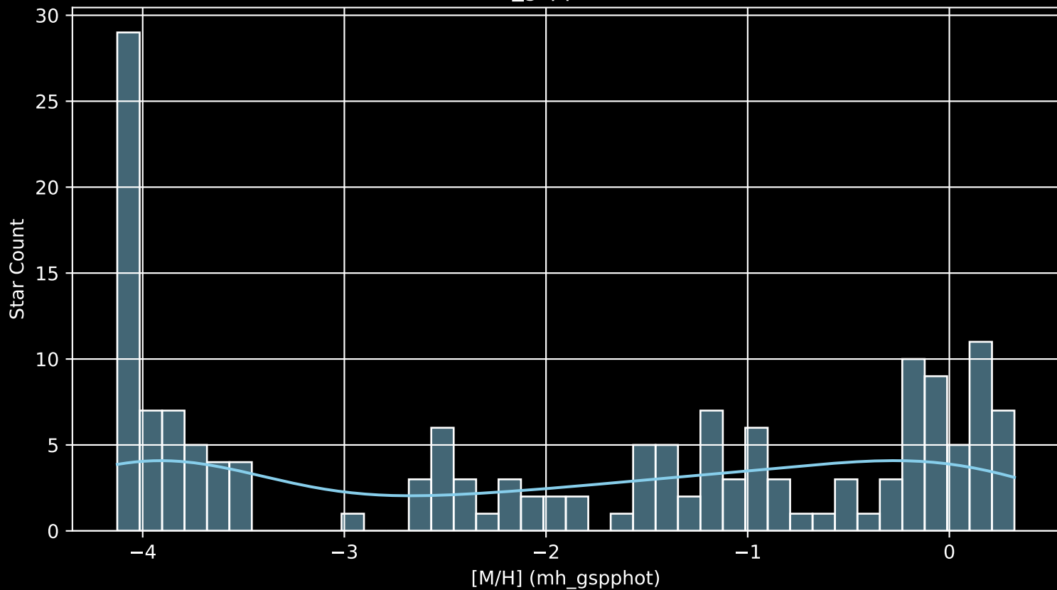
APOGEE DR17 Field: [356-06-O [M/H] (mh_gspphot) (n= 162)
